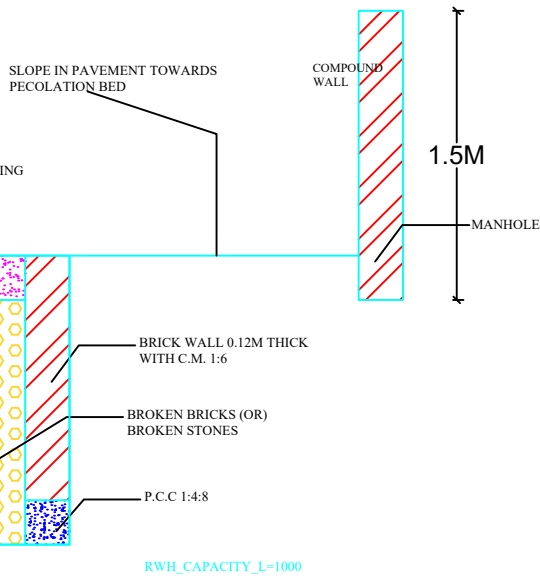
SECTION OF RAIN WATER PERCOLATION BED
