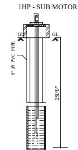
BOREWELL DETAILS
