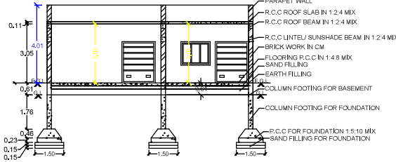
SECTION ON-AA
