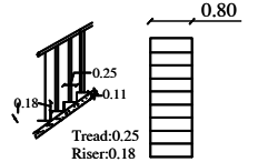
STAIRCASE DETAIL
