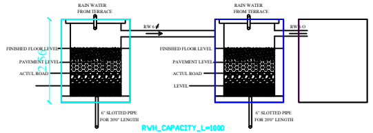
RAIN WATER COLL. TANK
