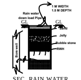
SEC. RAIN WATER HARVEST PIT
