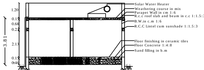
SECTION - "AB "
