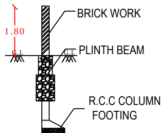
SECTION
