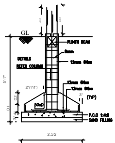
FOUNDATION DETAILS
