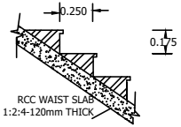
STAIR CASE STEPS SCALE 1:25
