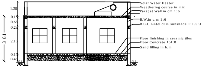
SECTION - "AB "
