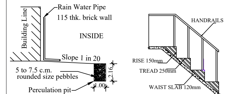
RAIN WATER HARVESTING PERCOLATION PIT
