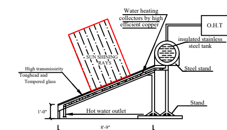
SECTION SOLAR WATER HEATER
