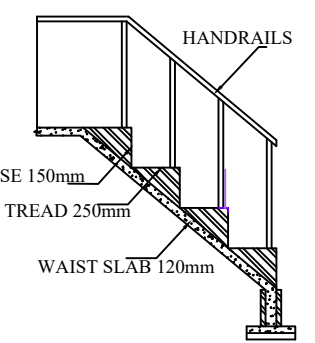
STAIRCASE DETAILS
