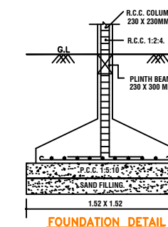
FOUNDATION DETAIL
