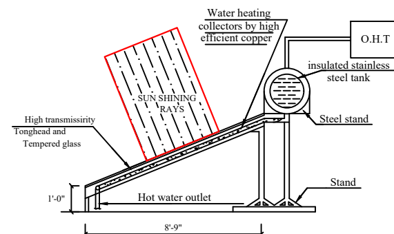
SECTION SOLAR WATER HEATER
