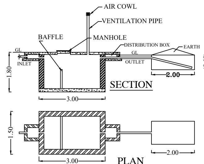
SEPTIC TANK DISPERSION TRENCH
