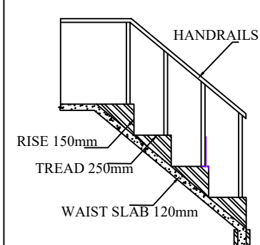
STAIRCASE DETAILS
