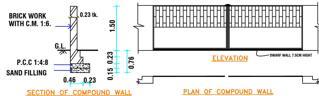
SECTION OF COMPOUND WALL
