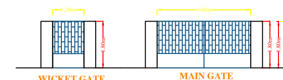
WICKET GATE
