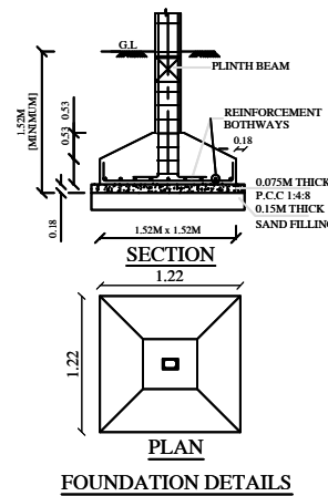
FOUNDATION DETAILS
