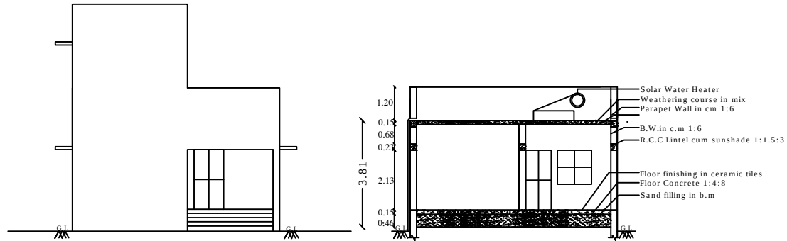
SECTION - "AB "
