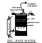
SEC. RAIN WATER HARVEST PIT
