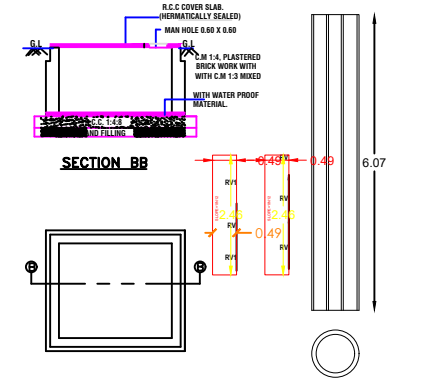
PLAN OF U.G. SUMP (CAPACITY = 12000 lt)
