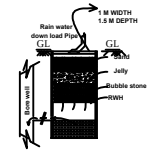
RAIN WATER COLLECTION TRENCH
