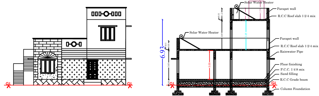
FRONT ELEVATION
