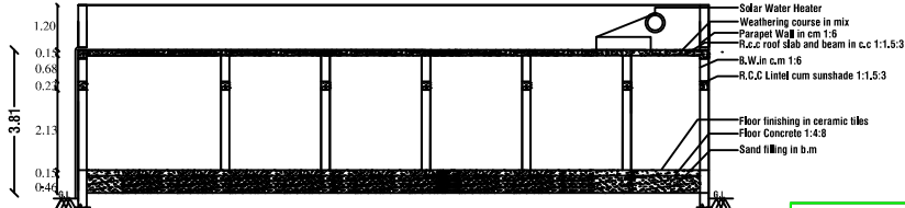
SECTION - "AB "
