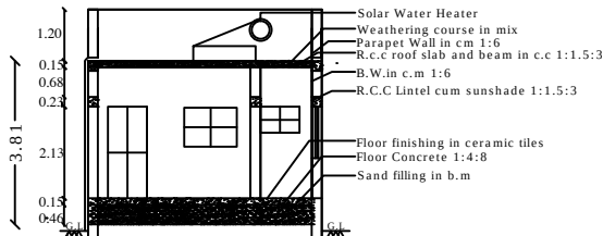
SECTION - "AB "
