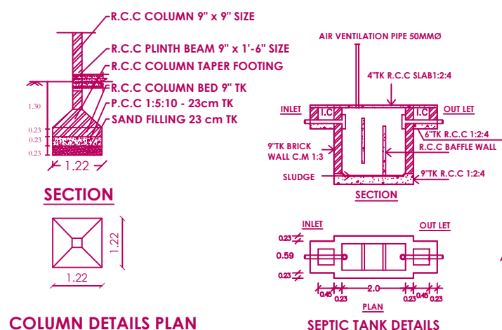
COLUMN DETAILS PLAN
