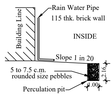
RAIN WATER HARVESTING PERCOLATION PIT
