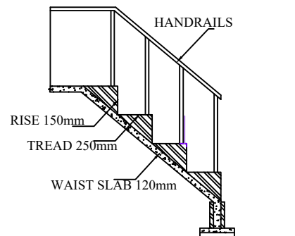
STAIRCASE DETAILS
