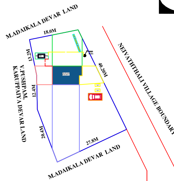
SITE PLAN
