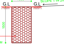
SECTION OF PEBBLE TRENCH SCALE : 1: = 100
