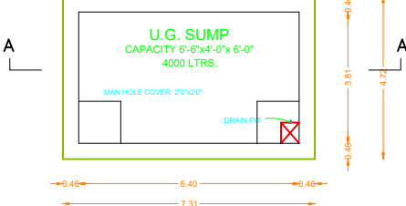
U.G. SUMP CAPACITY 6'-6"x4'-0"x 6'-0" 4000 LTRS.
