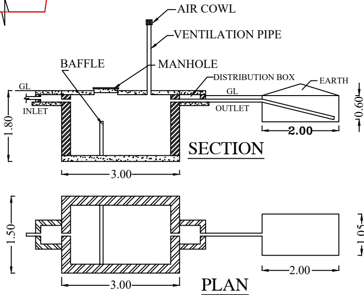
SEPTIC TANK DISPERSION TRENCH
