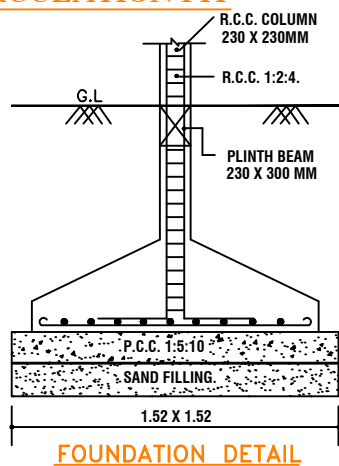
FOUNDATION DETAIL
