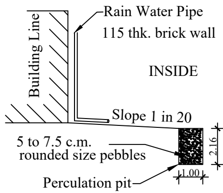
RAIN WATER HARVESTING PERCUSSION PIT
