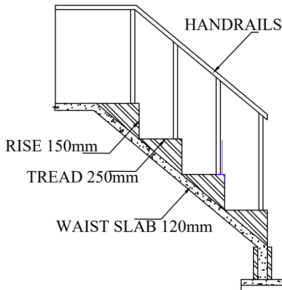
STAIRCASE DETAILS
