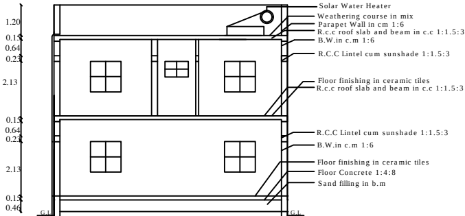
SECTION-"AB-CD "
