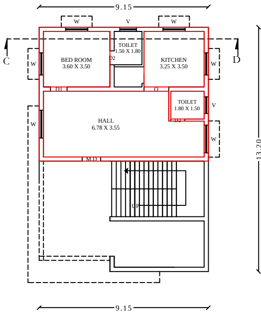
F FLOOR PLAN
