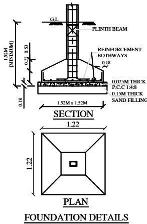
FOUNDATION DETAILS
