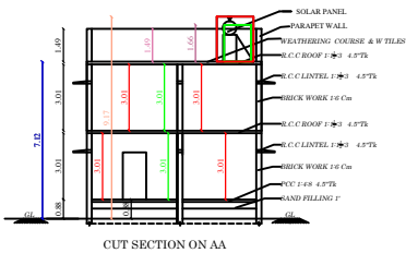
CUT SECTION ON AA
