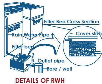
DETAILS OF RWH
