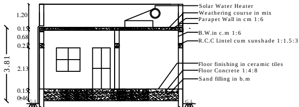
SECTION - "AB "
