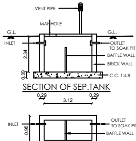
PLAN SEPTIC TANK
