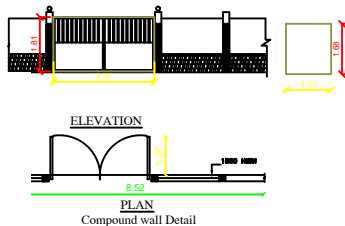
PLAN Compound wall Detail
