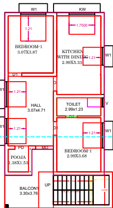
PROPOSED FIRST FLOOR PLAN
