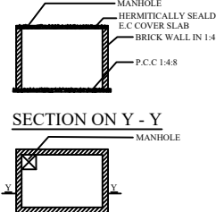
UG - SUMP DETAIL PLAN
