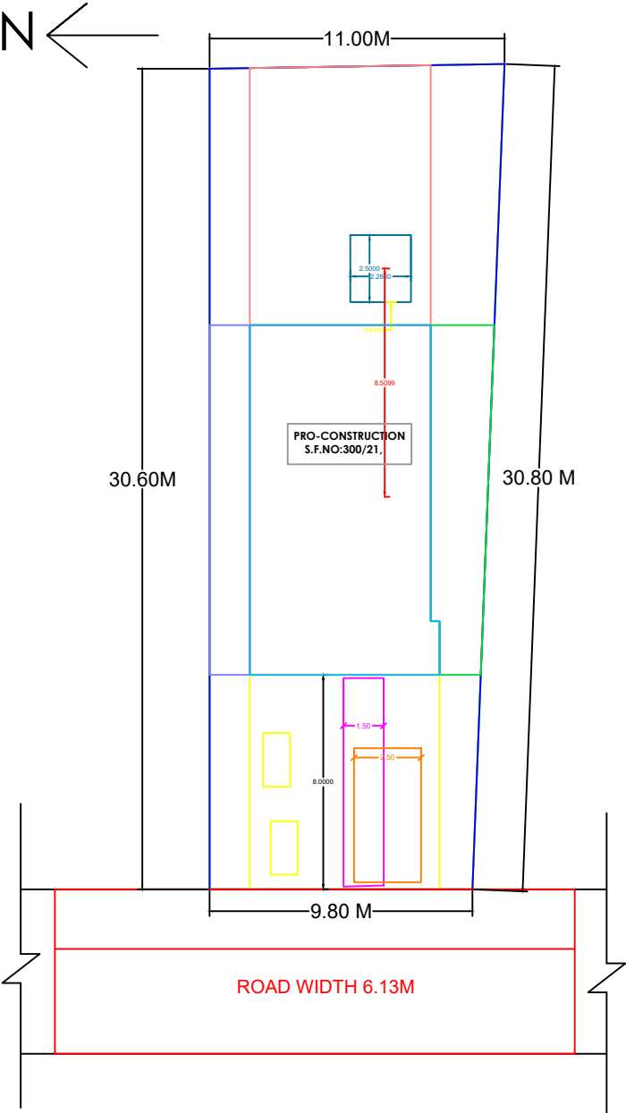
SITE PLAN-SCALE
