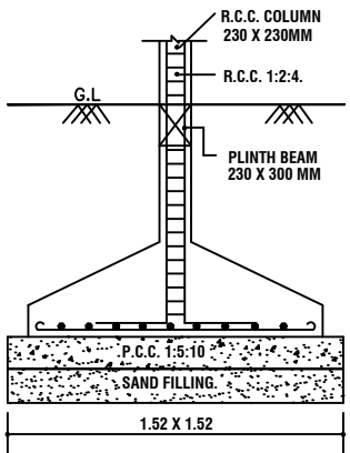
FOUNDATION DETAIL
