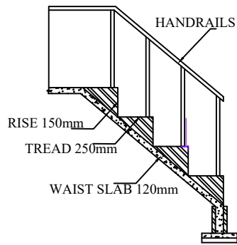
STAIRCASE DETAILS
