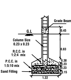
COLUMN DETAILS NOT TO SCALE
