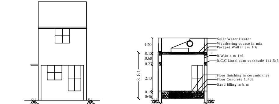
SECTION - "AB "
