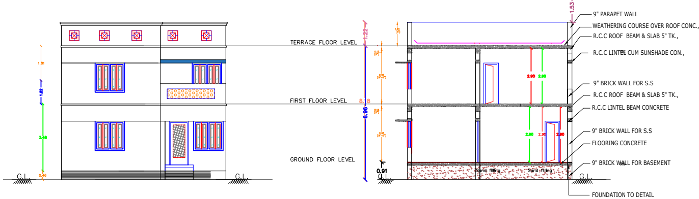
FRONT ELEVATION
