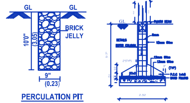
FOUNDATION DETAILS
