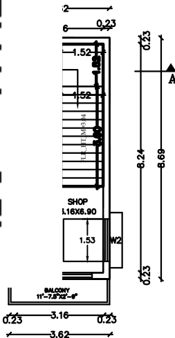
FRIST FLOOR PLAN
