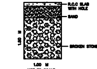
RAIN WATER HARVEST COLLECTION PIT.
