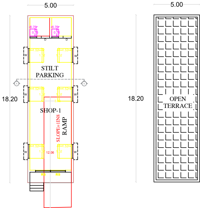
BASEMENT FLOOR CUM GROUND FLOOR PLAN SCALE 1:100
