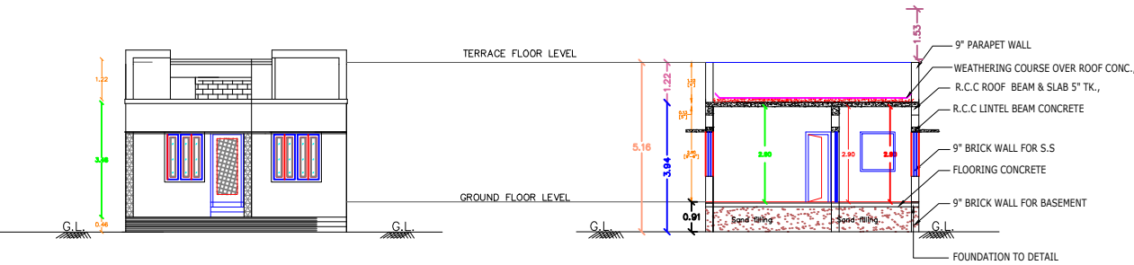
FRONT ELEVATION
