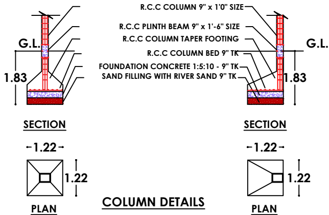
COLUMN DETAILS
