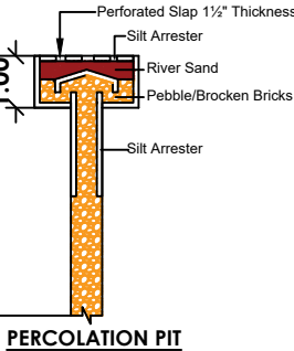
PERCOLATION PIT
