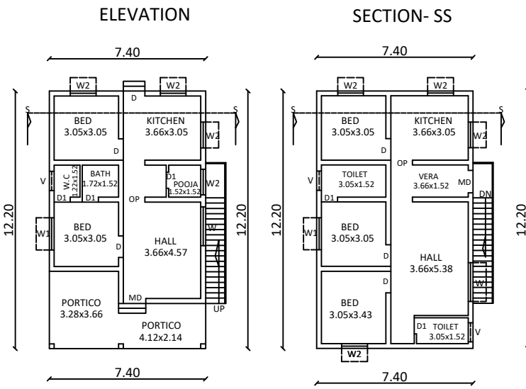
(EXG) GROUND FLOOR PLAN (PRO) FIRST FLOOR PLAN
