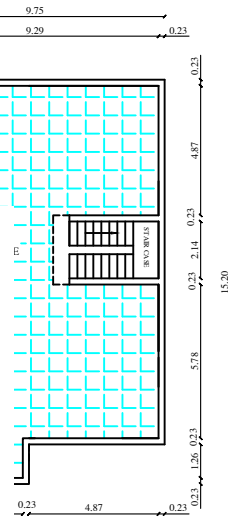
FLOOR PLAN
