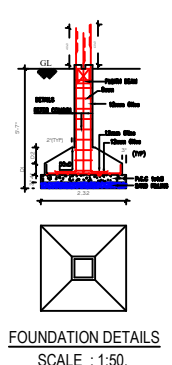
FOUNDATION DETAILS SCALE : 1:50
