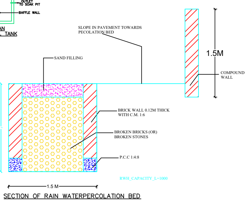
SECTION OF RAIN WATERPERCOLATION BED
