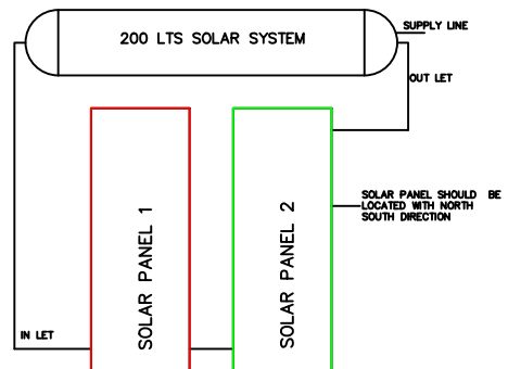
SOLAR WATER HEATER SYSTEM
