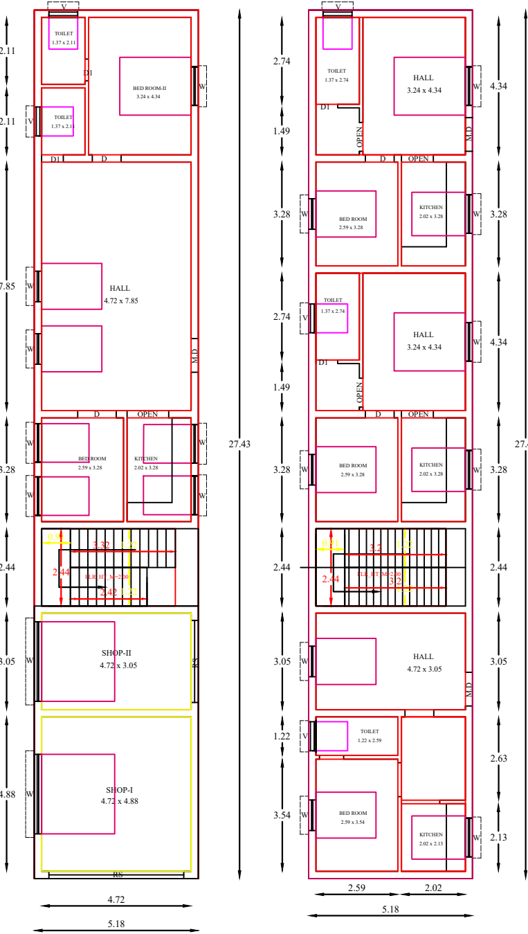
GROUND FLOOR PLAN SCALE 1: 100 FIRST FLOOR PLAN SCALE 1: 100
