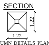
COLUMN DETAILS PLAN
