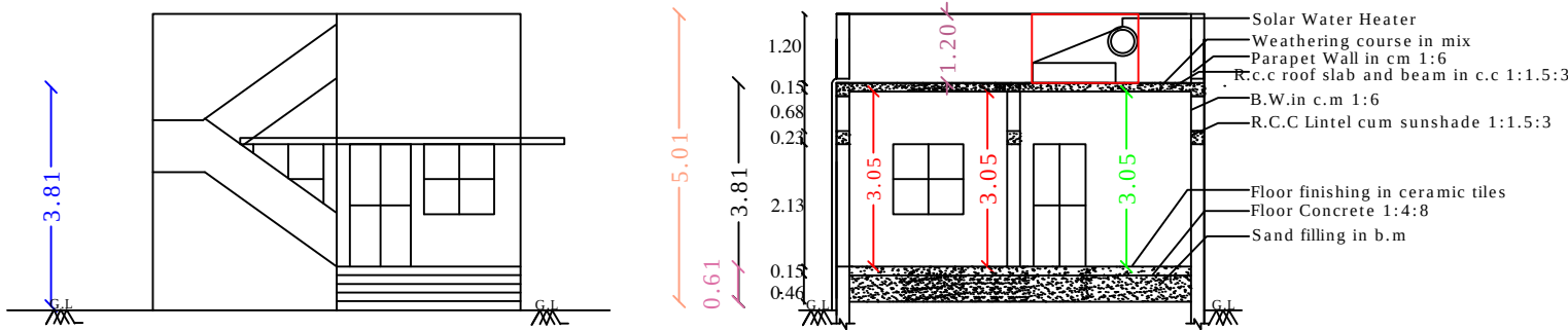
SECTION - "AB "
