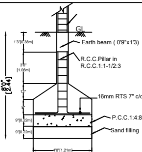
FOUNDATION DETAILS
