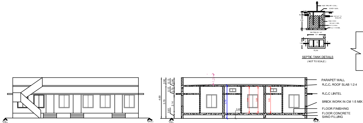
SECTION A1-A1
