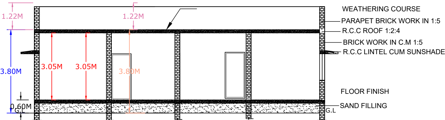
SECTION ON XX
