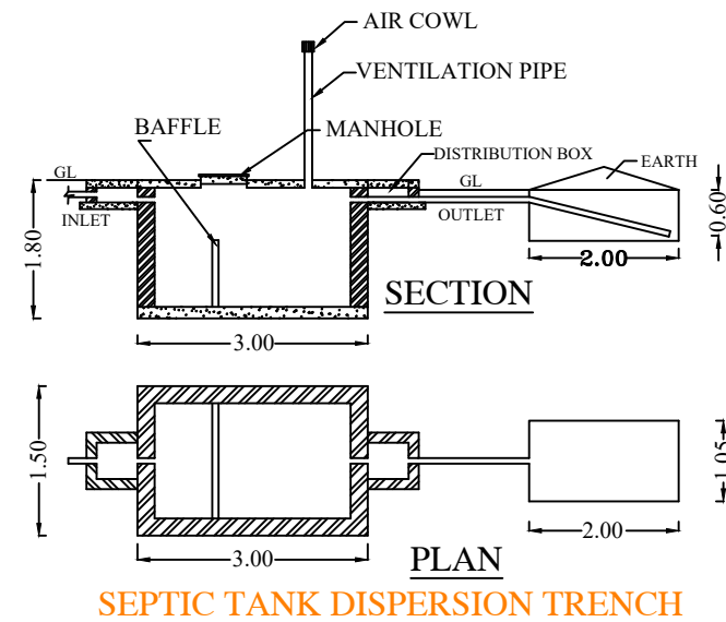
SEPTIC TANK DISPERSION TRENCH
