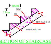
SECTION OF STAIRCASE
