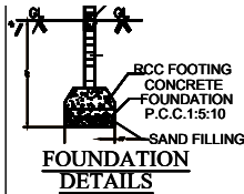
FOUNDATION DETAILS
