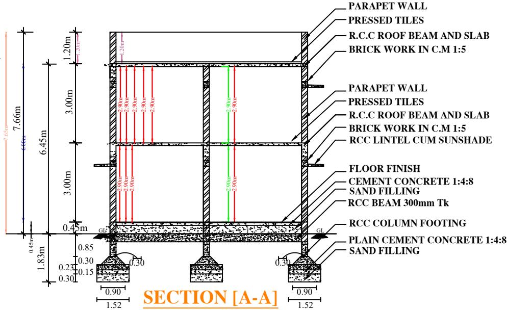
SECTION [A-A]
