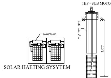
BOREWELL DETAILS
