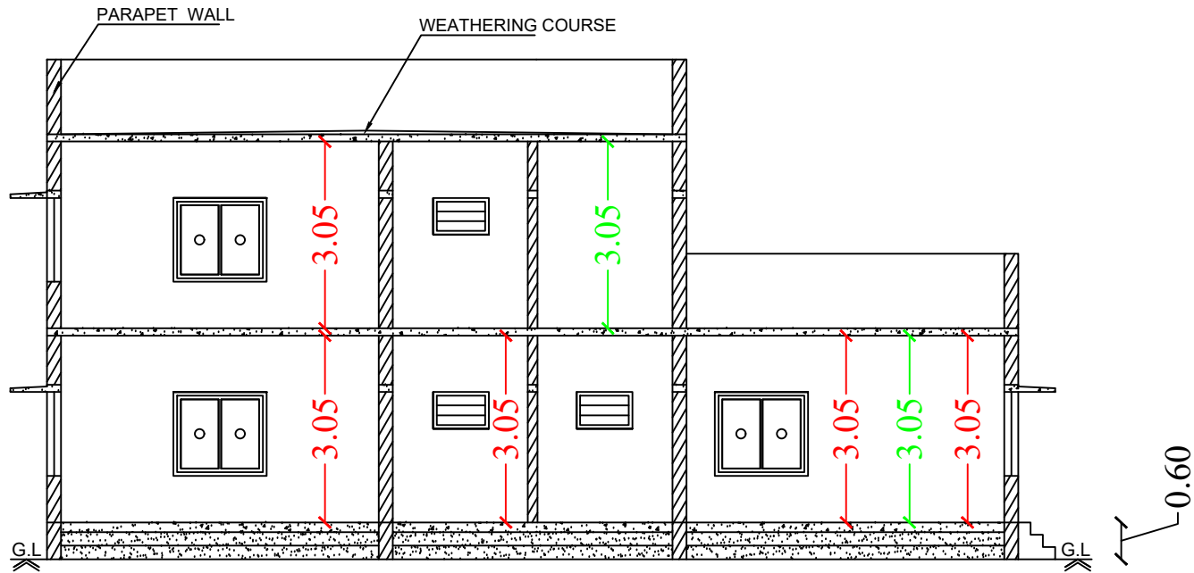
Section on-"AA"
