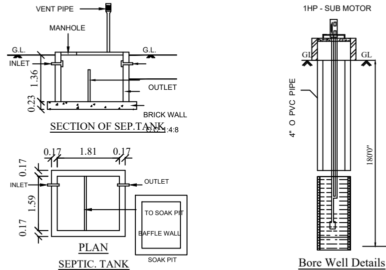
SEPTIC TANK
