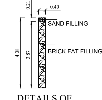
DETAILS OF PERCULATION PIT
